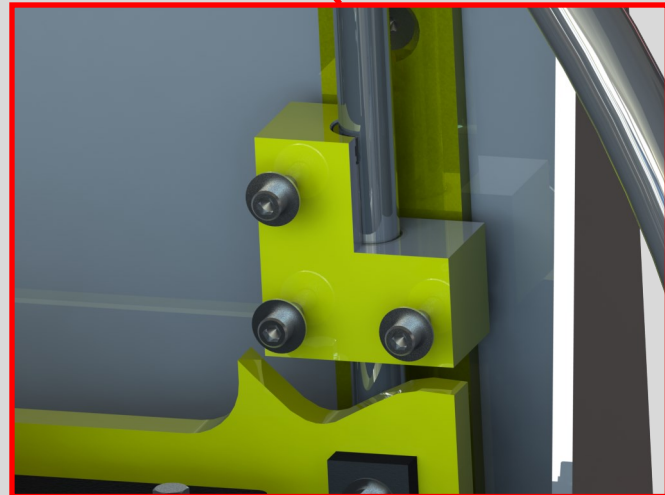
Upgraded Plain Bearing and Rod style Rail shown. (Cutaway shown for clarity)
